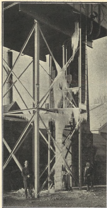
ICICLES EXTRAORDINARY. The pipes leading to and from a 20,000 gallon tank at the Orchard Factory, Toddington, burst during the severe frost, and the dripping water covered the approach ladder and stays with a sheet of ice.
