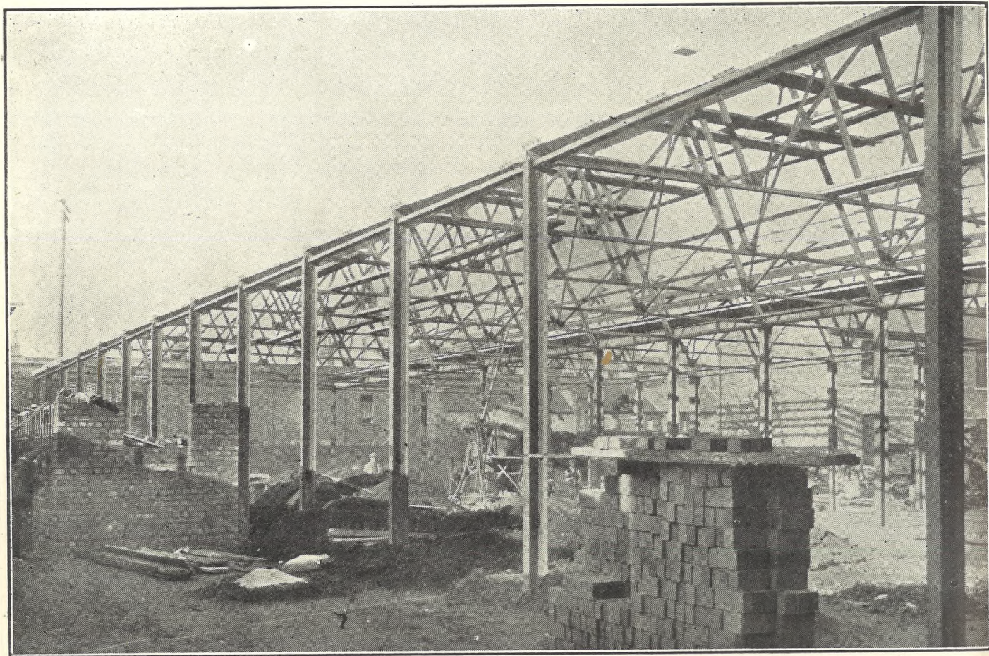
STEEL SKELETON IN COURSE OF ERECTION, AND PREPARATIONS FOR MACHINE BEDS.
