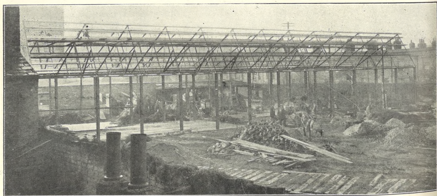
THE ROOF BEGINS TO TAKE SHAPE. NOTE MODERN MIXING MACHINES.
