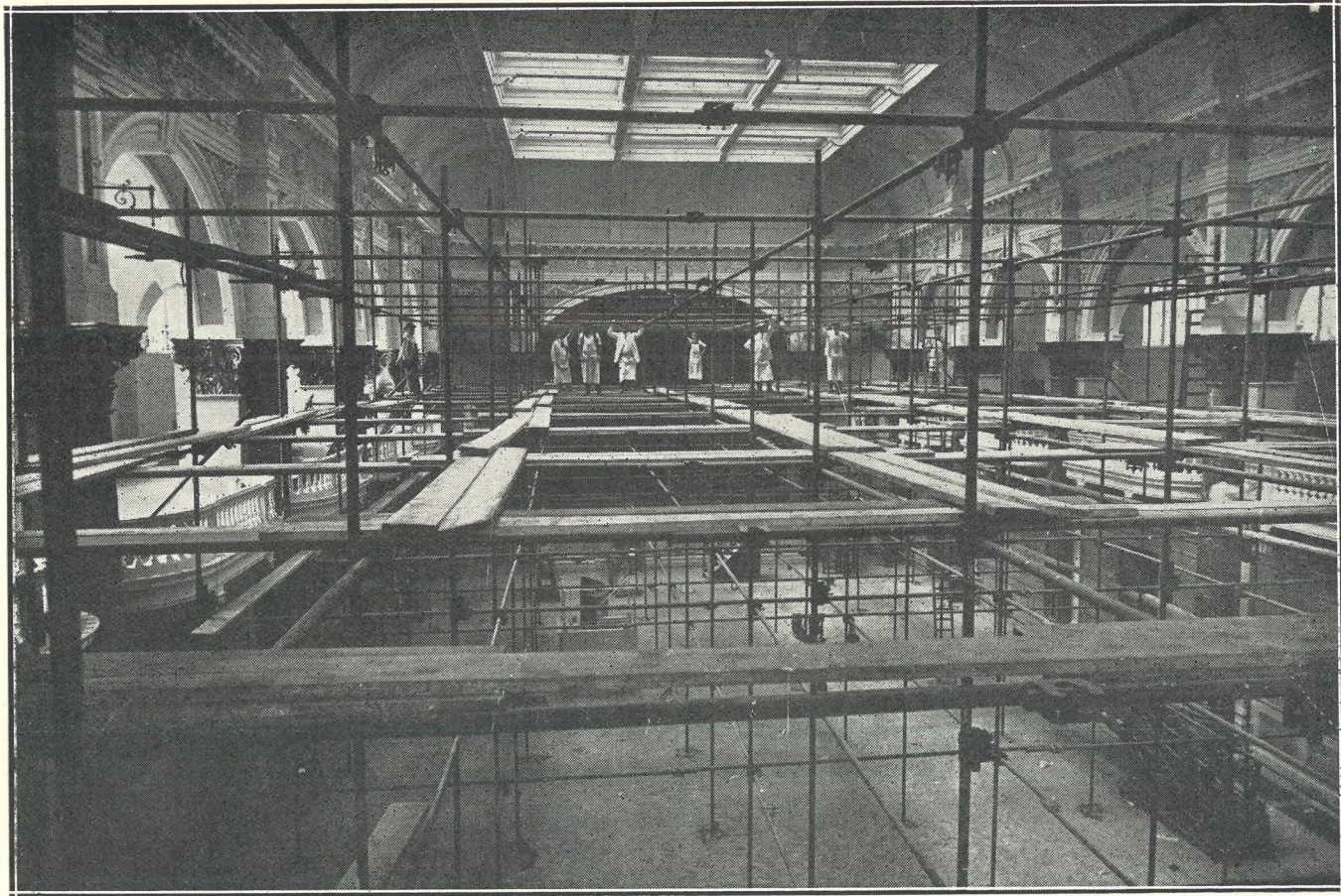
The Town Hall, Cheltenham, during the course of Redecoration by Messrs. Conway Jones & Co., Ltd., of Gloucester. This photograph was taken whilst the men were at work on the special tubular scaffolding. Photo by W. Slatter.
