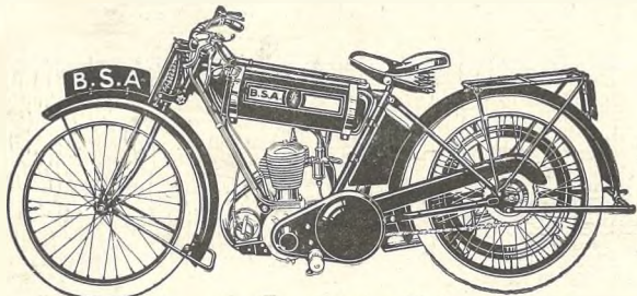
249 H.P. 4-Stroke, 2-Speed, Clutch, Kick-start, Mech. Oil Pump, Adjustable Handlebars and Footrests. 35 Gns.
