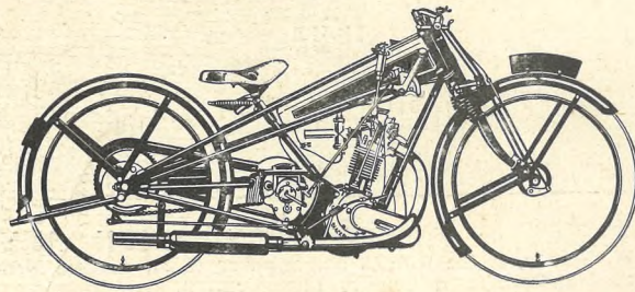
2½ H.P. O.H.V., Large Port T.T. Engine. All-chain drive, 3-speed gear, clutch & kickstarter £64-10s.
