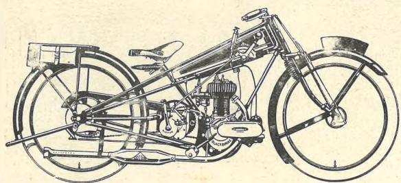
2½ H.P. Side Valve Model. All-chain drive, 3-speed gear, clutch and kickstarter £56-15s.
