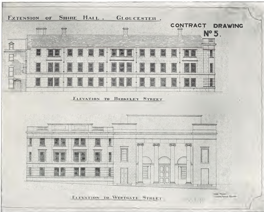
ELEVATIONS OF NEW WING.
